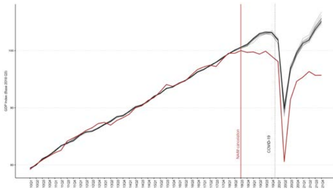
(a) Leave-one-out
